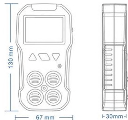
Size : 130x67x30mm
