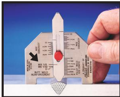
CHECK REINFORCEMENT
